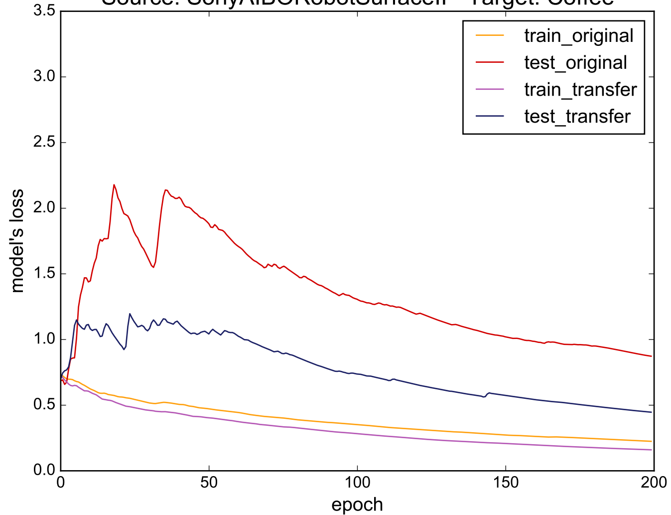
Source: SonyAIBORobotSurfacell - Target: Coffee
