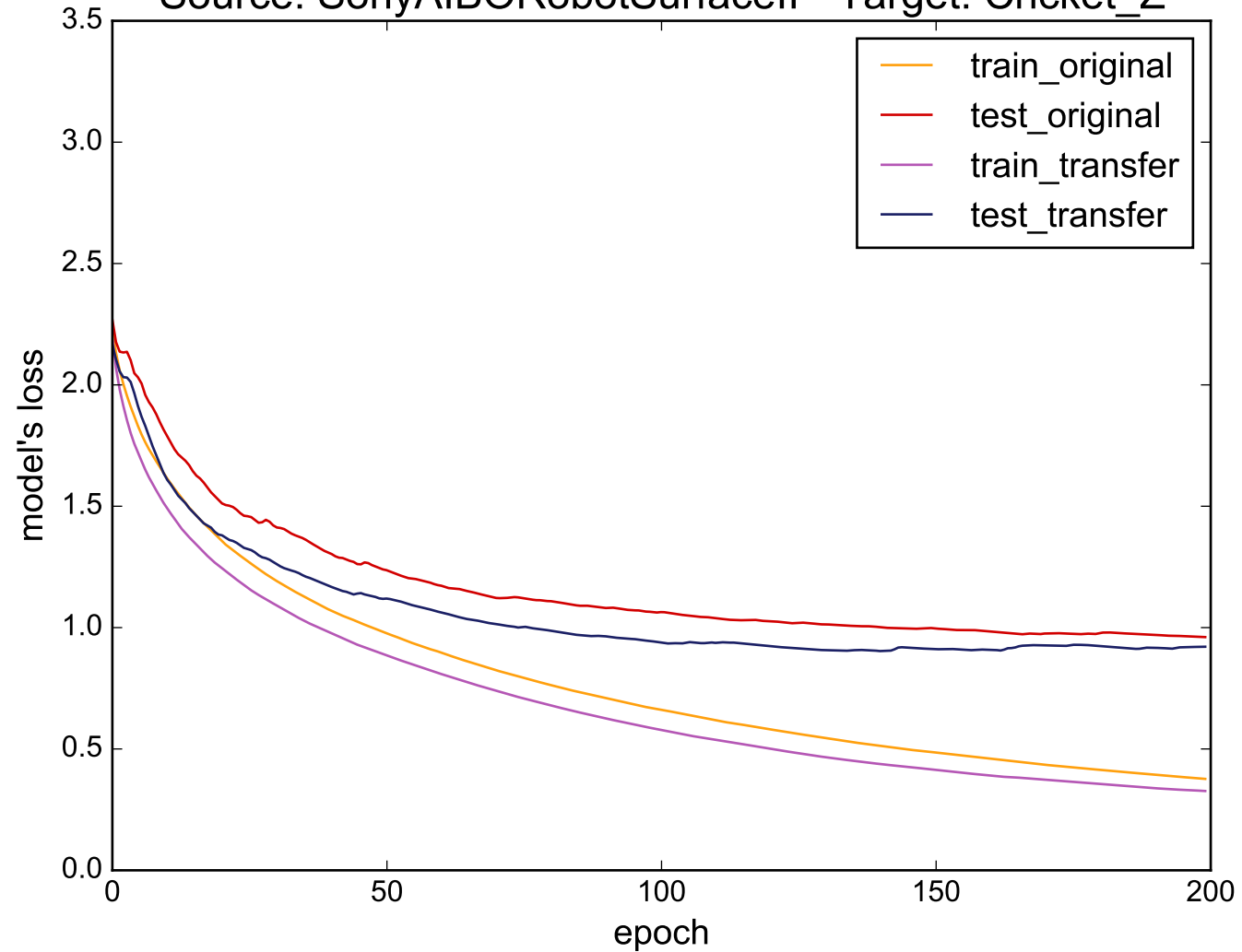
Source: SonyAIBORobotSurfaceII - Target: Cricket_Z
