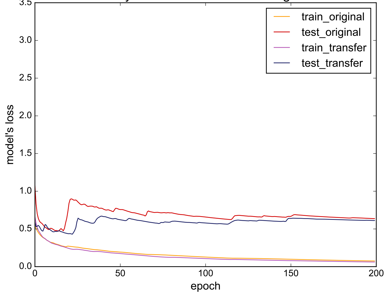
Source: SonyAIBORobotSurfaceII - Target: ECG200
