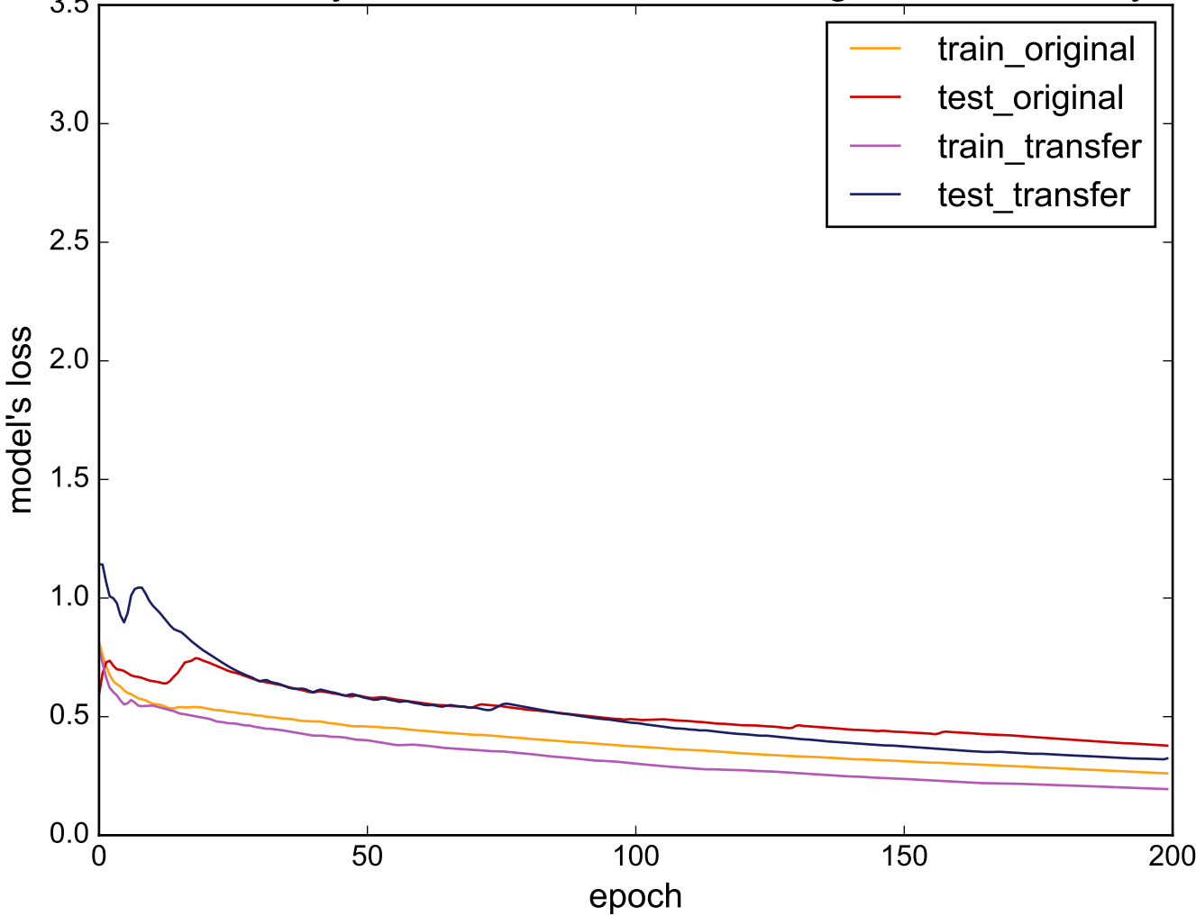
Source: SonyAIBORobotSurfacell - Target: ECGFiveDays
