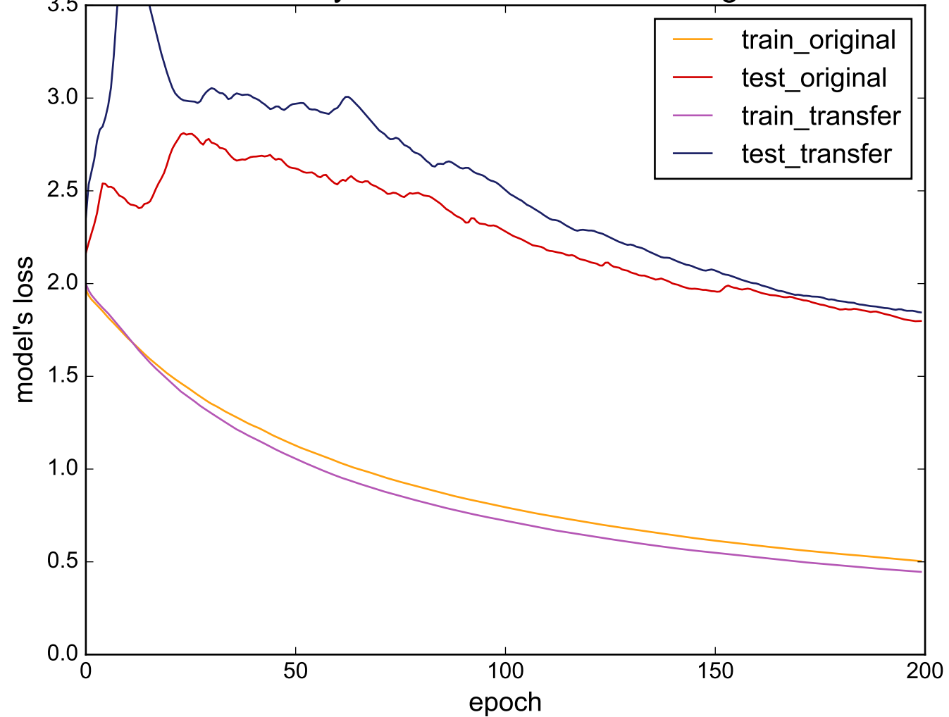
Source: SonyAIBORobotSurfacell - Target: FISH
