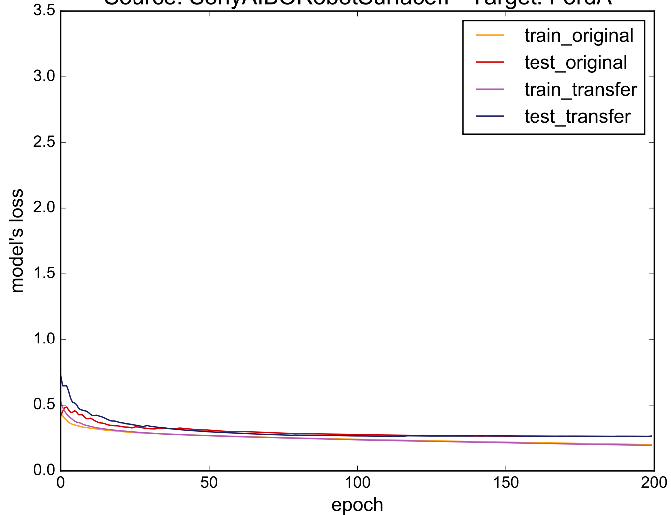
Source: SonyAIBORobotSurfaceII - Target: FordA
