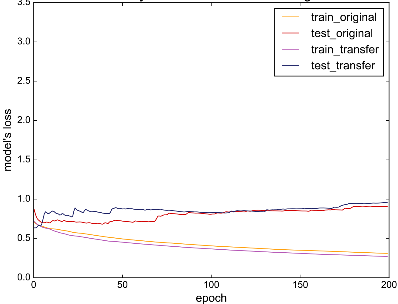
Source: SonyAIBORobotSurfacell - Target: Ham
