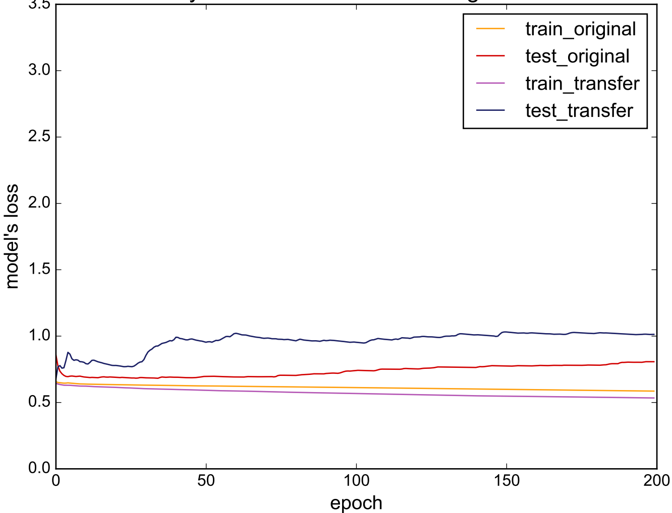
Source: SonyAIBORobotSurfacell - Target: HandOutlines
