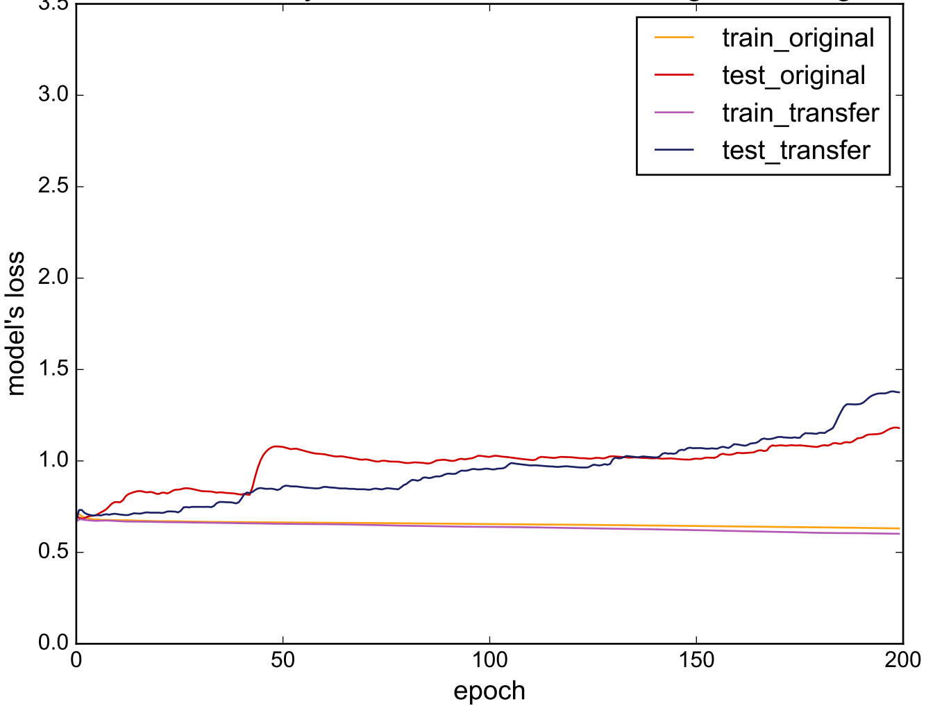
Source: SonyAIBORobotSurfcell - Target: Herring
