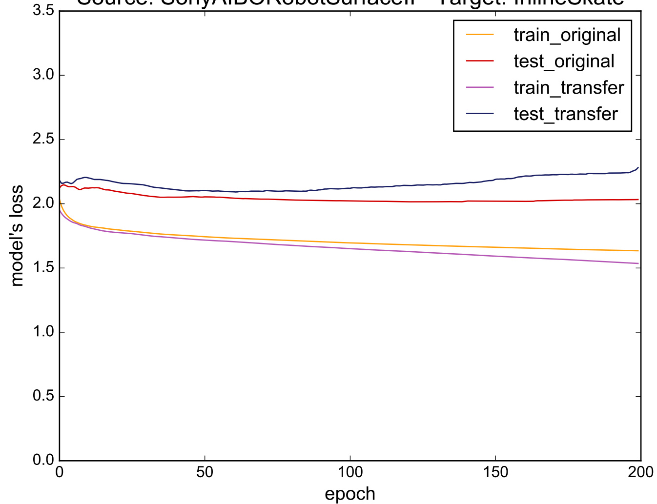
Source: SonyAIBORobotSurfacell - Target: InlineSkate
