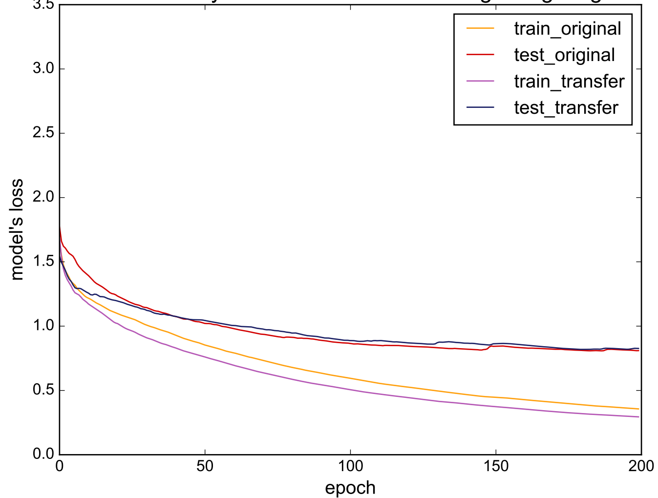
Source: SonyAIBORobotSurfaceII - Target: Lighting7
