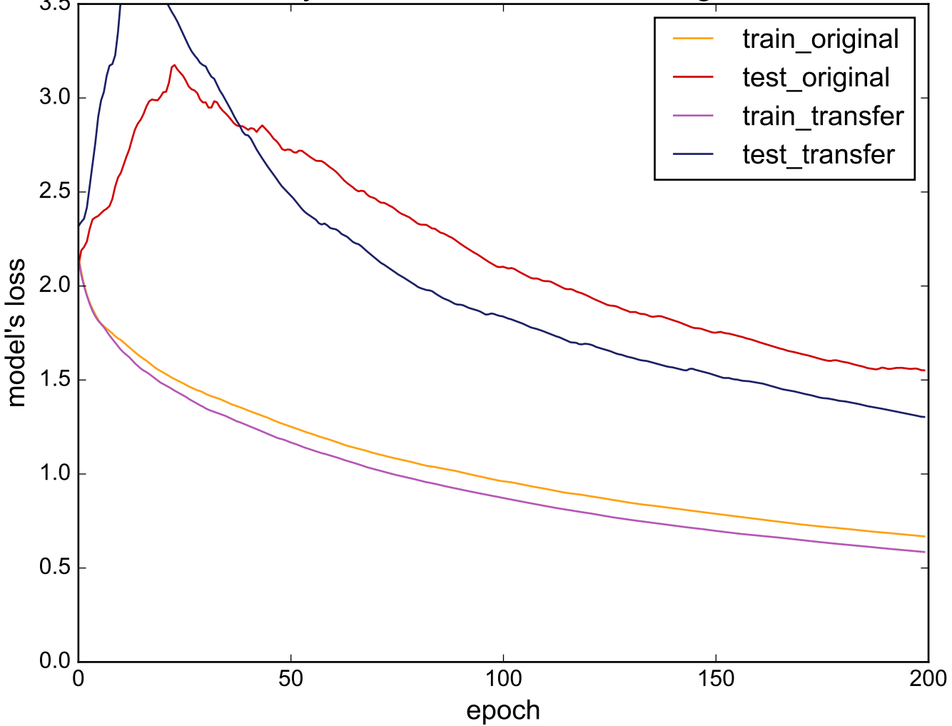
Source: SonyAIBORobotSurfaceII - Target: MALLAT
