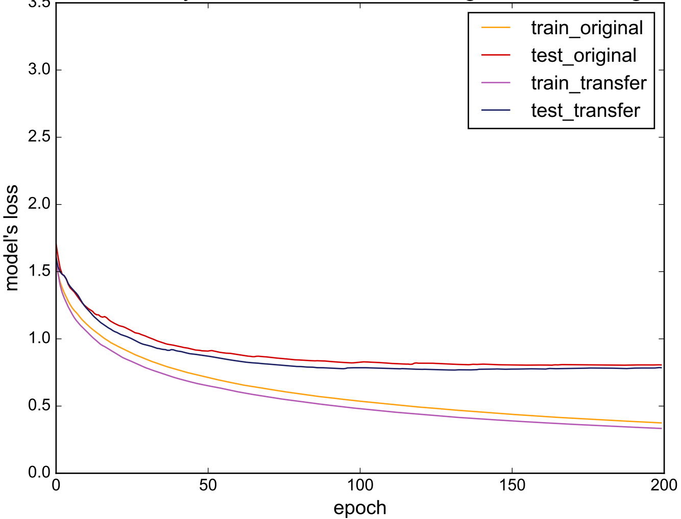
Source: SonyAIBORobotSurfaceII - Target: MedicalImages
