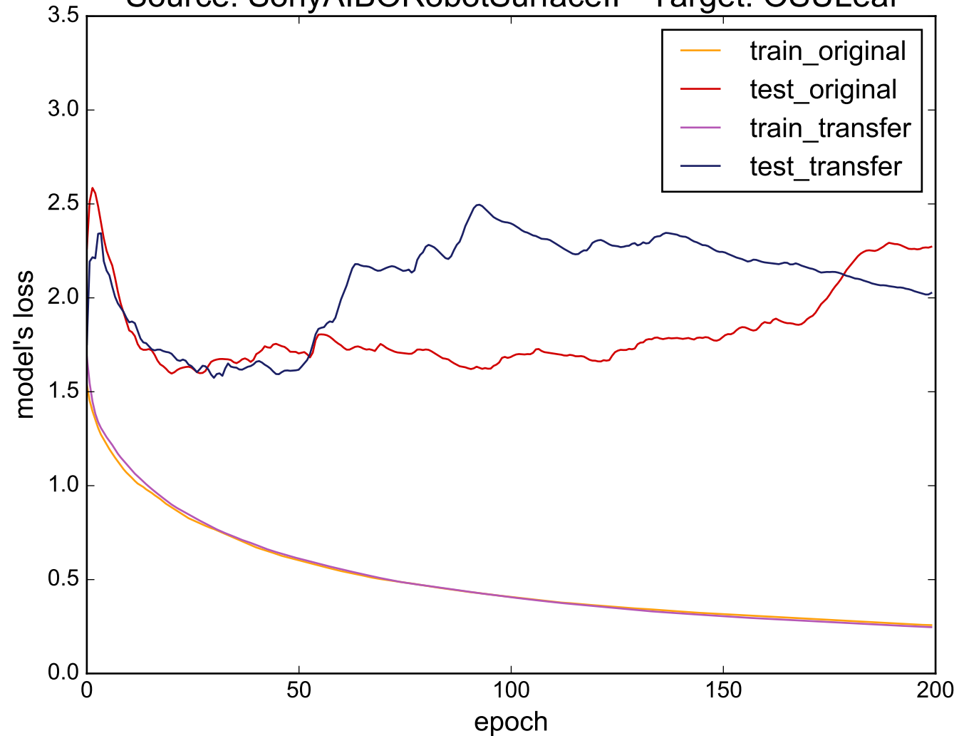
Source: SonyAIBORobotSurfacecell - Target: OSULeaf
