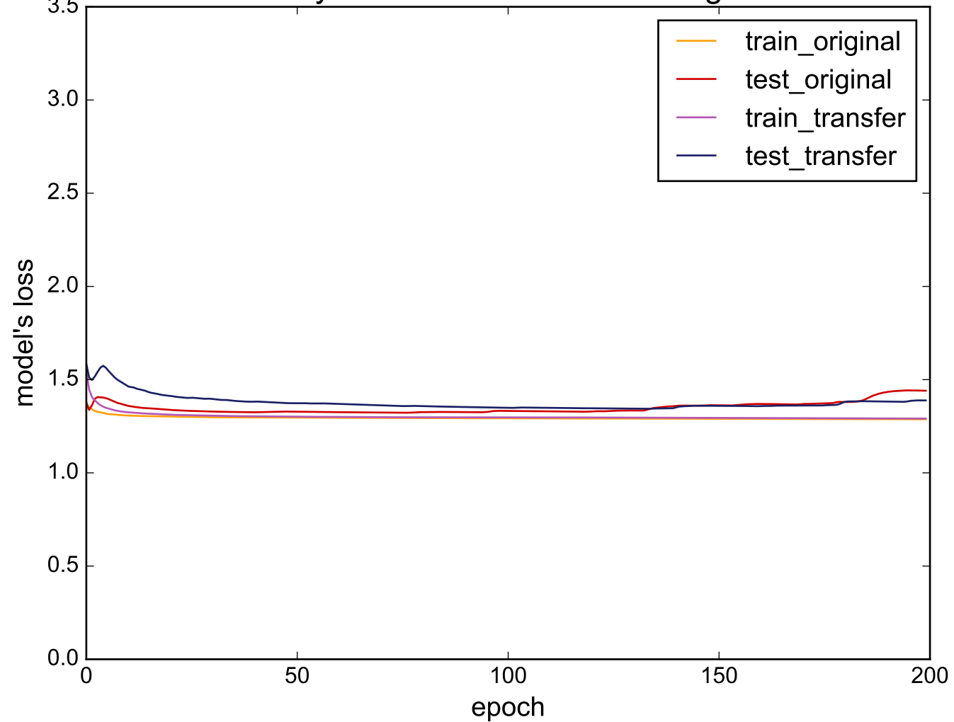
Source: SonyAIBORobotSurfacell - Target: OliveOil
