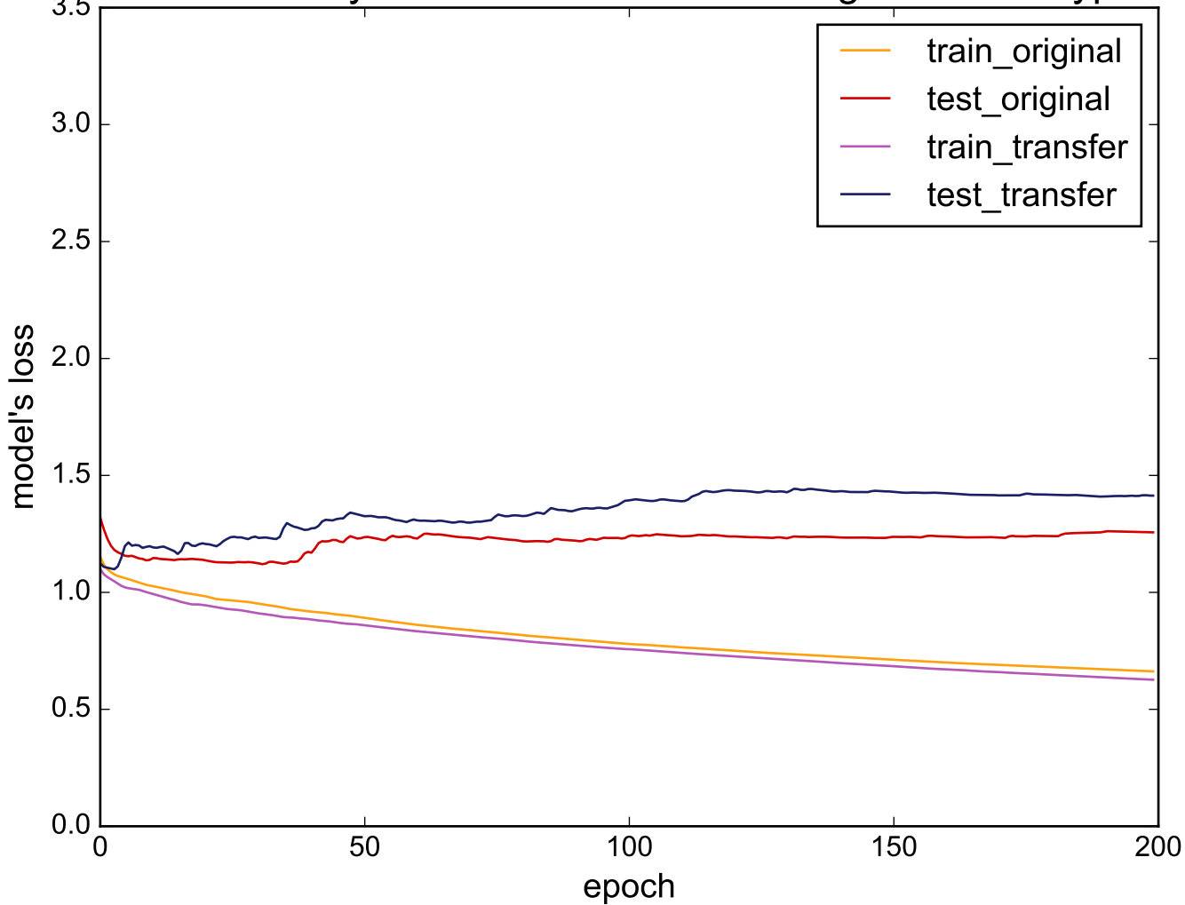
Source: SonyAIBORobotSurfaceII - Target: ScreenType
