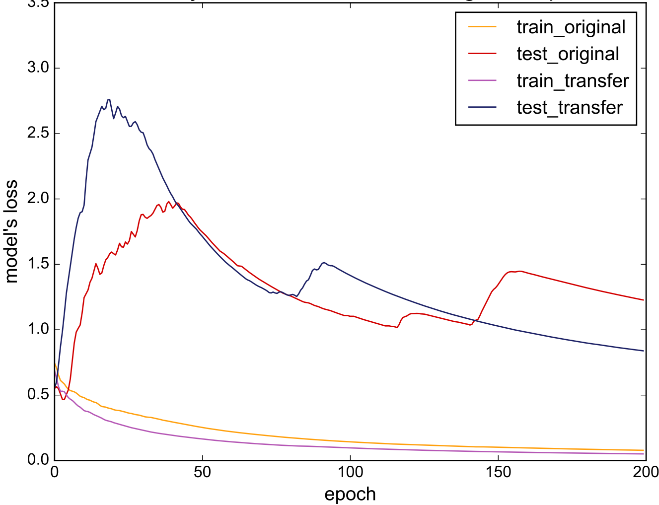
Source: SonyAIBORobotSurfaceII - Target: ShapeletSim
