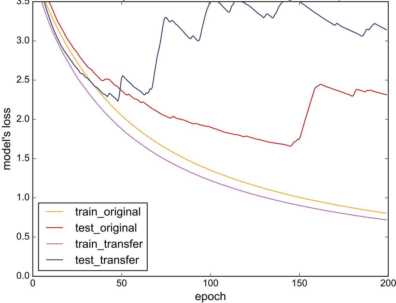
Source: SonyAIBORobotSurfacell - Target: ShapesAll
