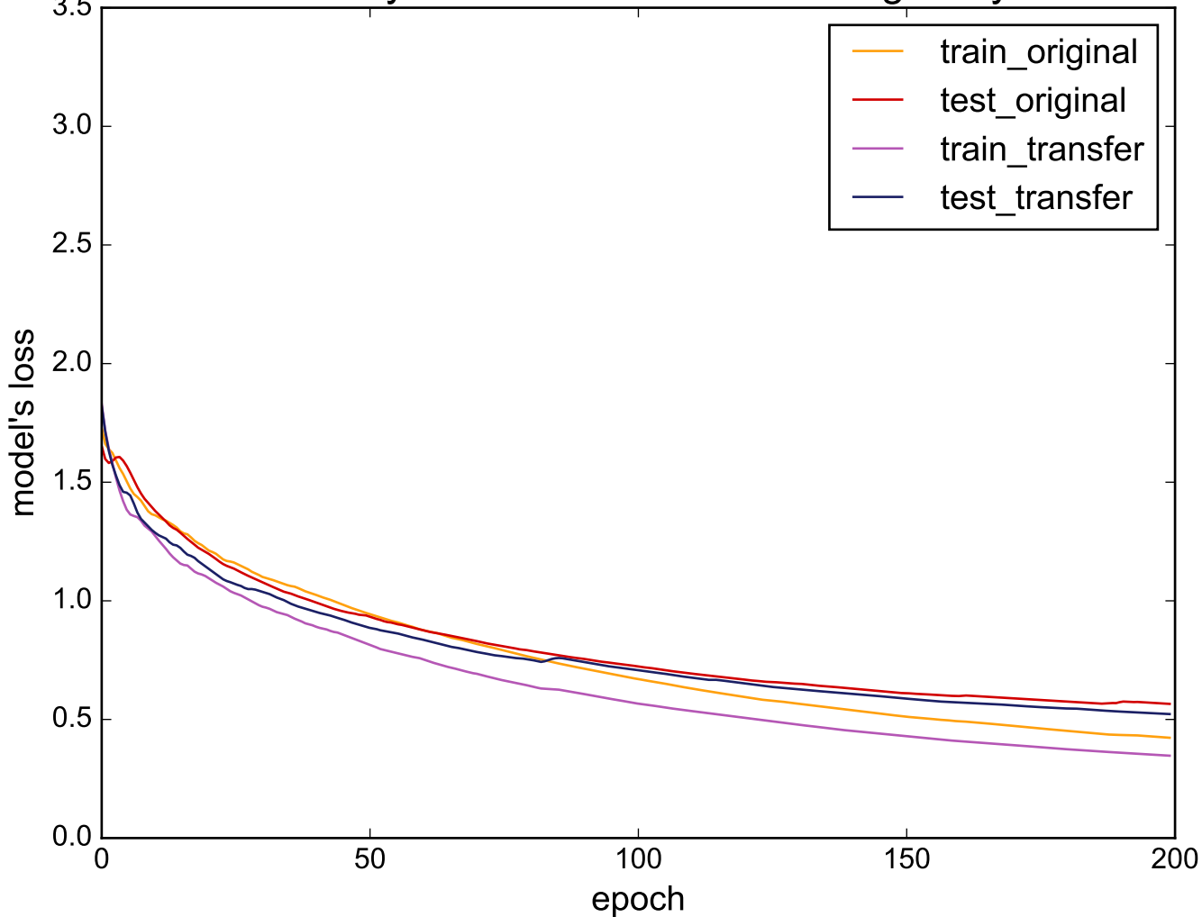
Source: SonyAIBORobotSurfaceII - Target: Symbols
