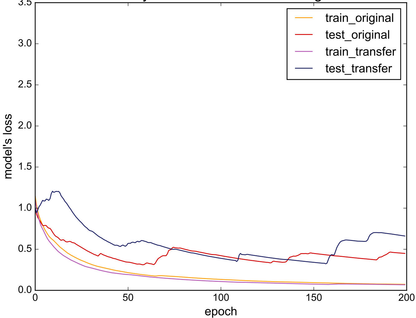
Source: SonyAIBORobotSurfaceII - Target: Trace
