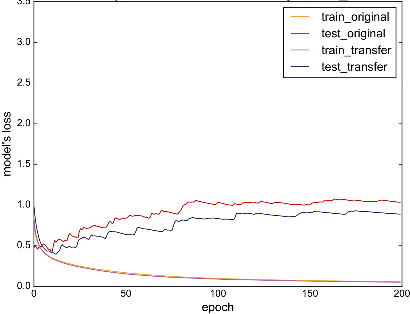
Source: SonyAIBORobotSurfacell - Target: Two_Patterns
