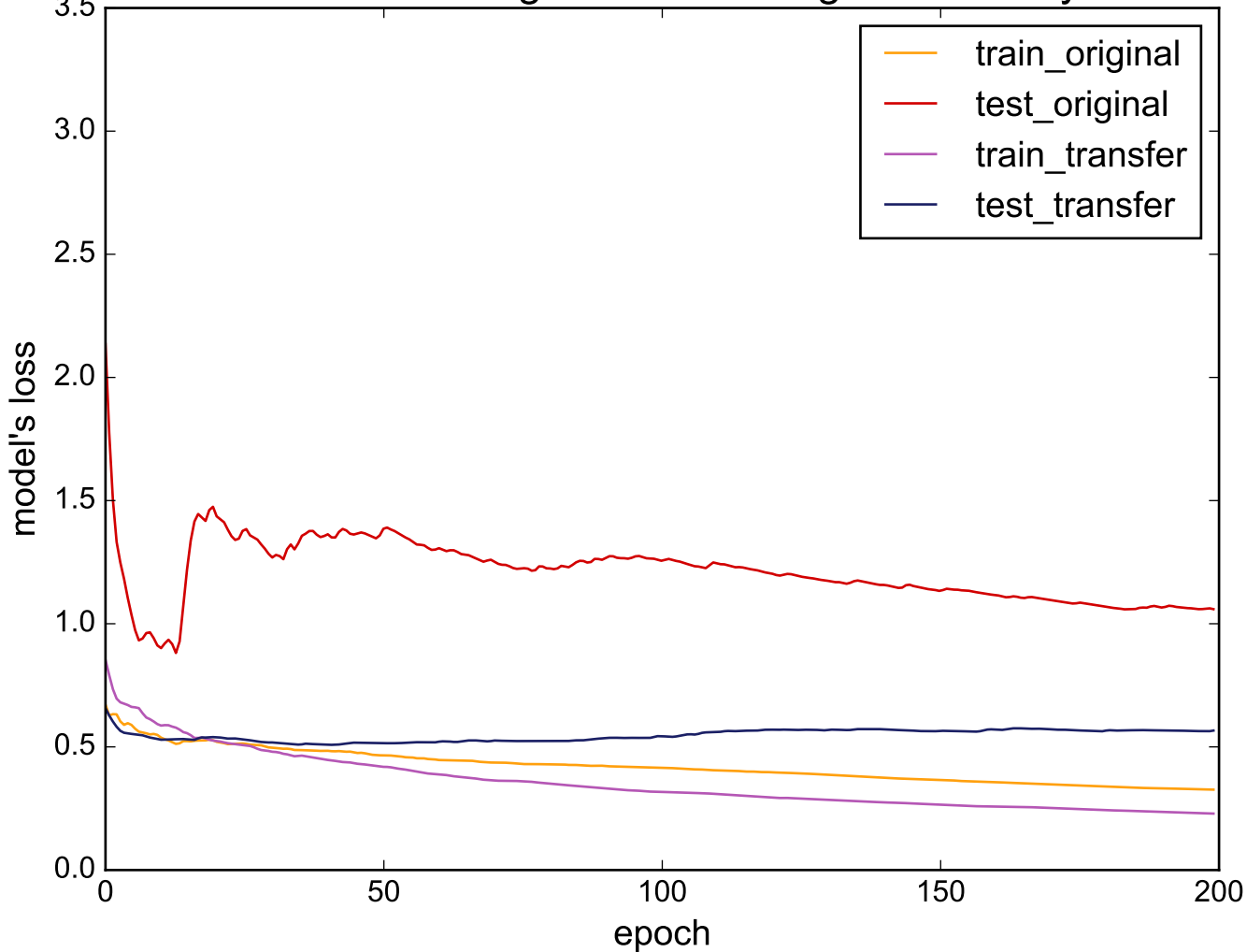
Source: StarLightCurves - Target: BeetleFly
