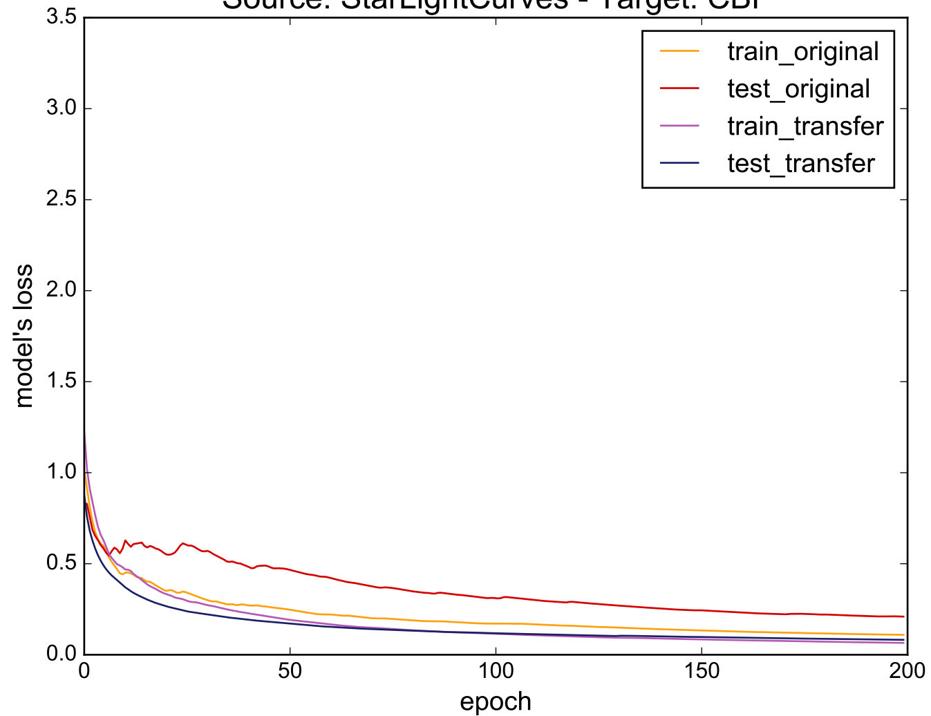
Source: StarLightCurves - Target: CBF
