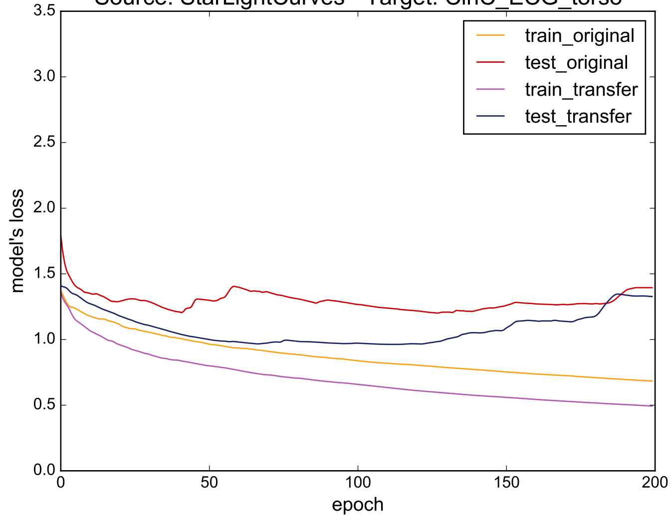
Source: StarLightCurves - Target: CinC_ECG_torso
