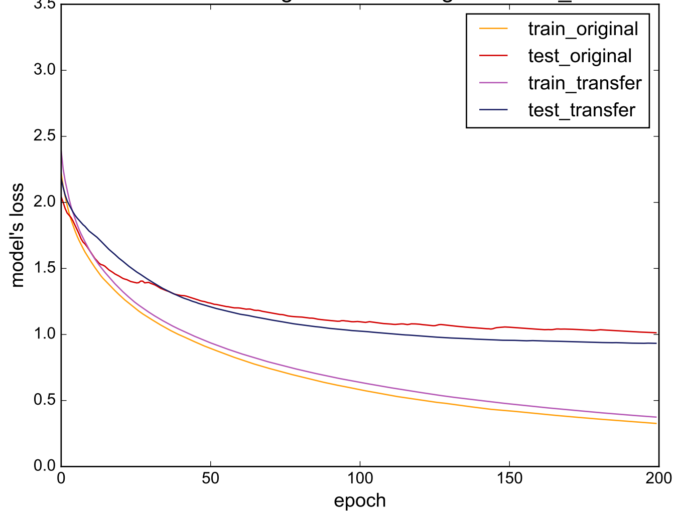
Source: StarLightCurves - Target: Cricket_X
