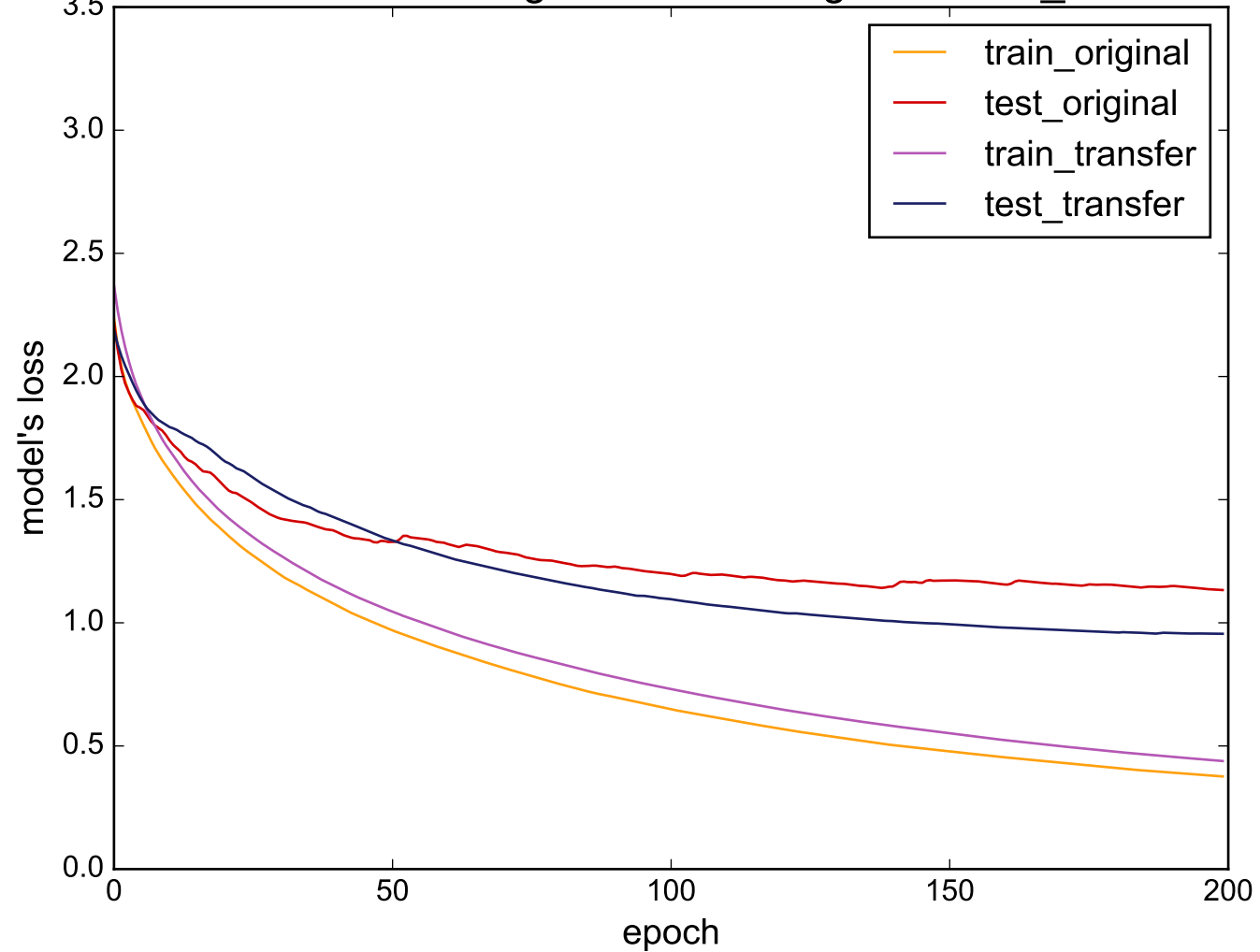
Source: StarLightCurves - Target: Cricket_Y
