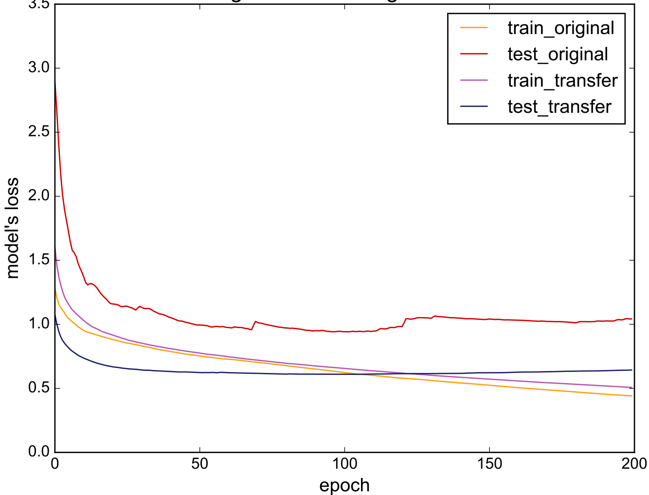
Source: StarLightCurves - Target: DistalPhalanxTW
