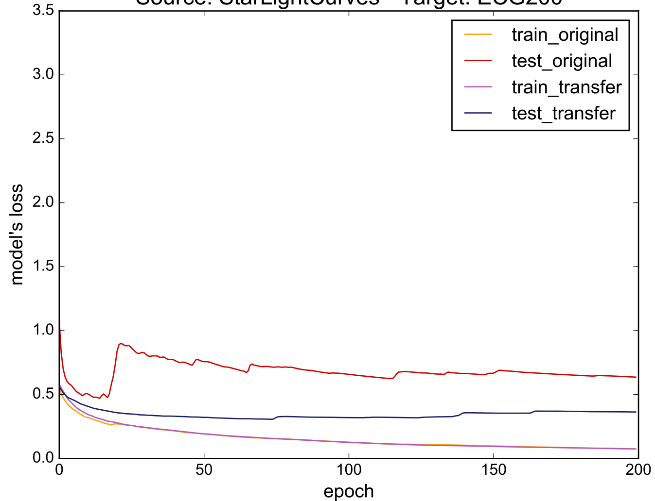
Source: StarLightCurves - Target: ECG200
