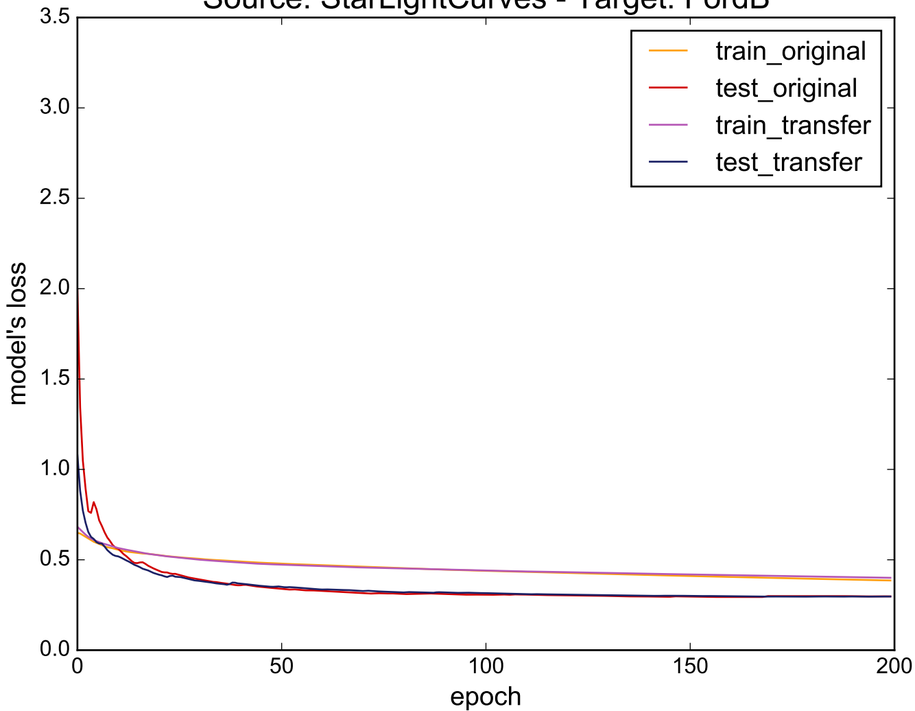
Source: StarLightCurves - Target: FordB
