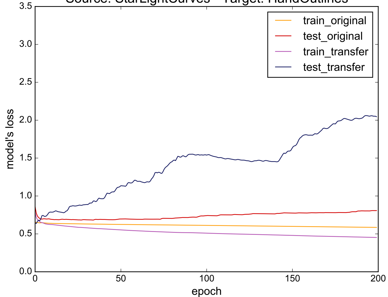
Source: StarLightCurves - Target: HandOutlines
