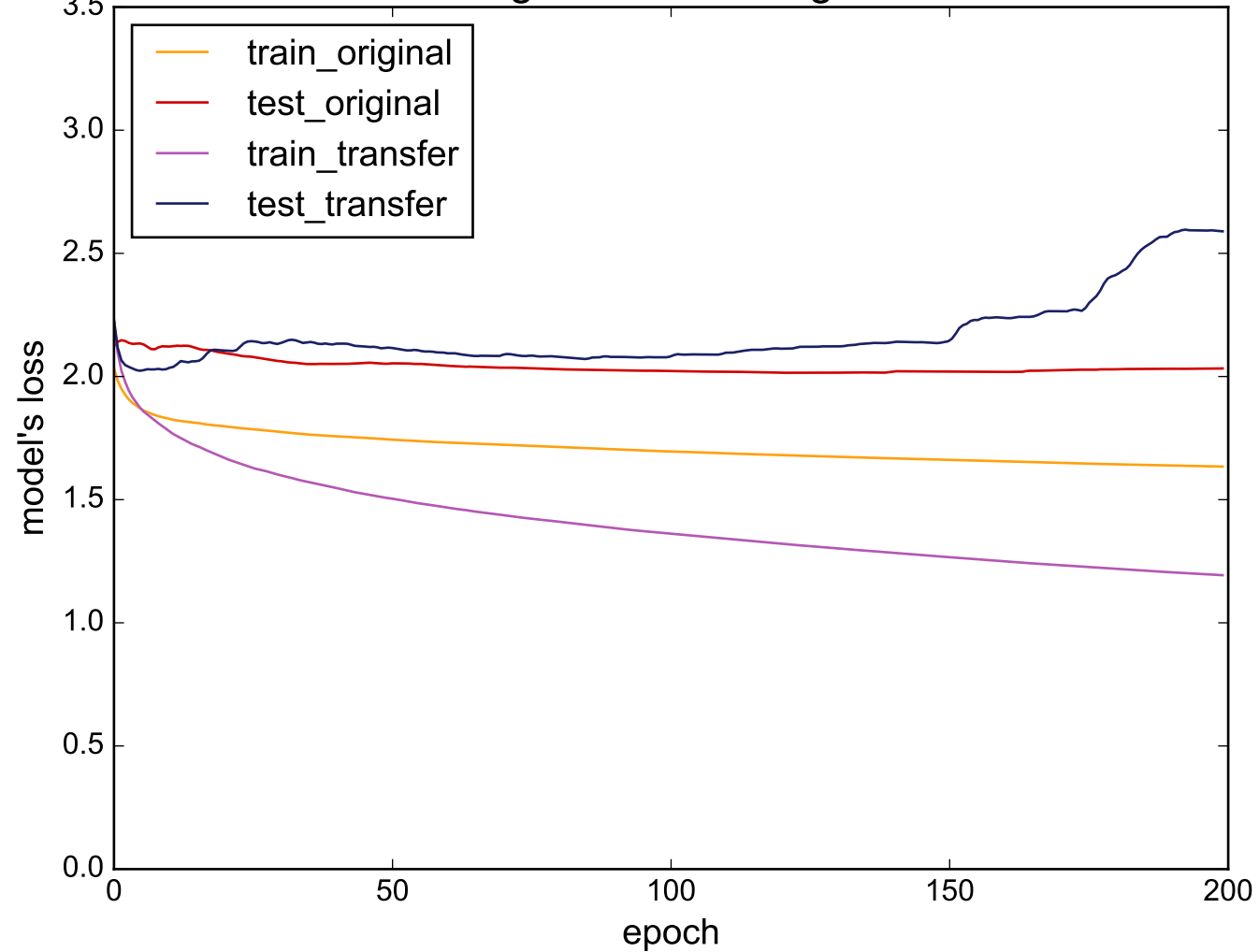
Source: StarLightCurves - Target: InlineSkate
