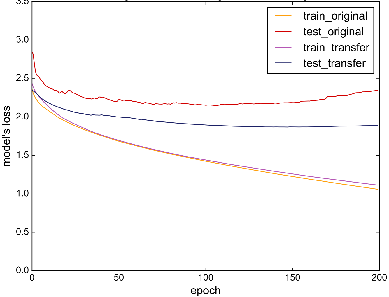
Source: StarLightCurves - Target: InsectWingbeatSound
