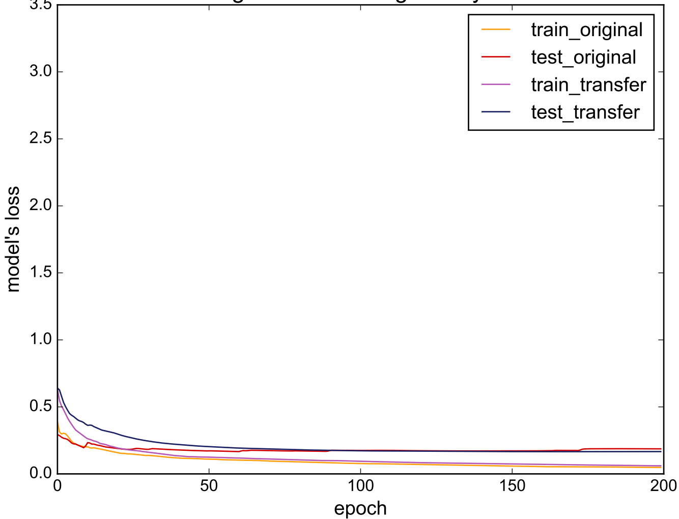
Source: StarLightCurves - Target: ItalyPowerDemand
