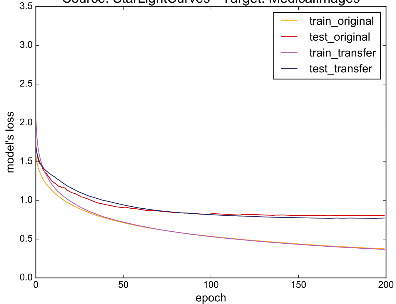
Source: StarLightCurves - Target: MedicalImages
