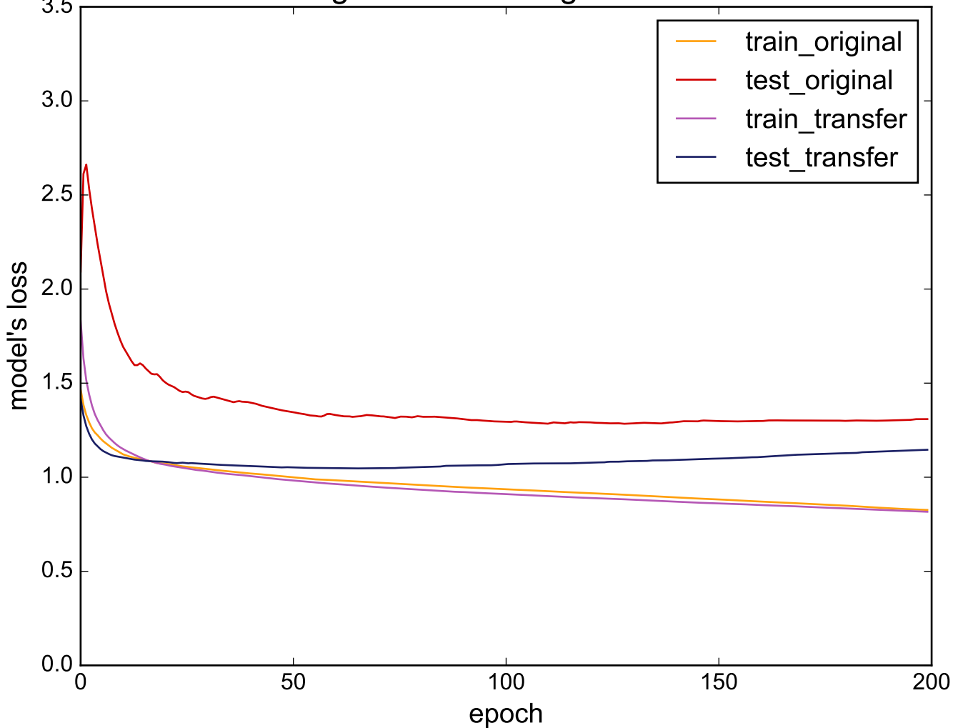
Source: StarLightCurves - Target: MiddlePhalanxTW
