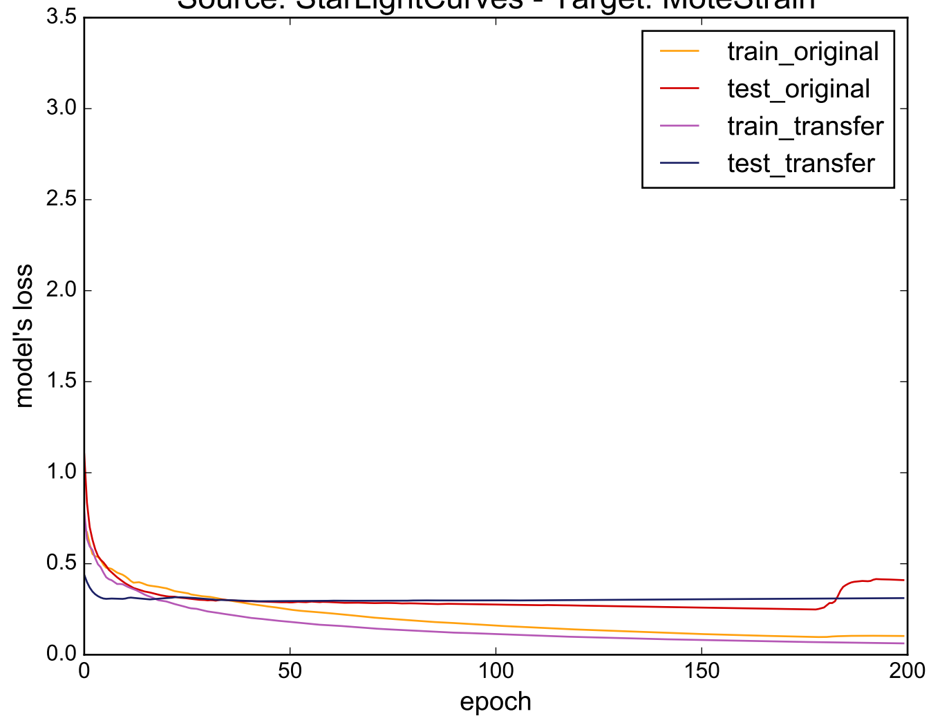
Source: StarLightCurves - Target: MoteStrain
