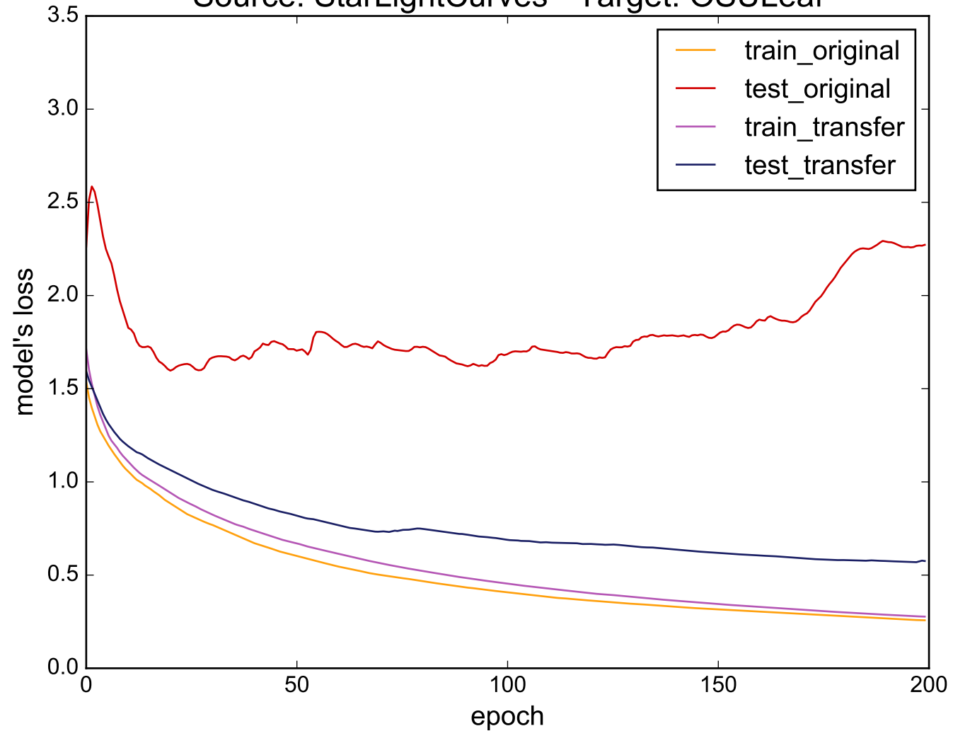
Source: StarLightCurves - Target: OSULeaf
