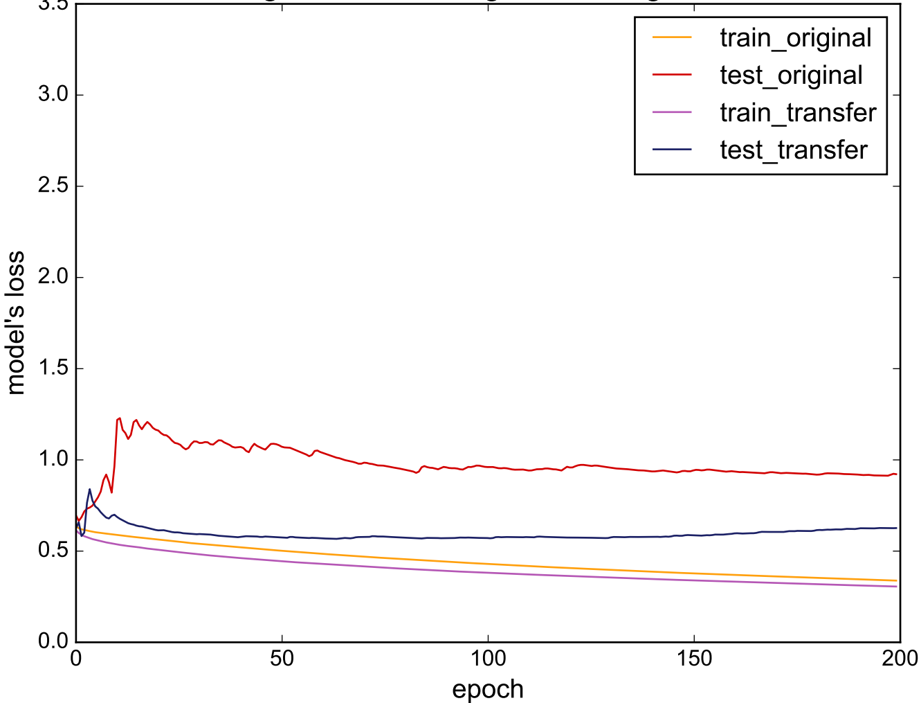
Source: StarLightCurves - Target: PhalangesOutlinesCorrect
