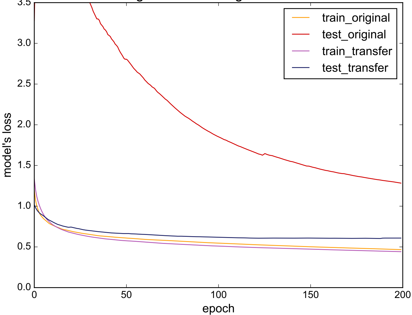
Source: StarLightCurves - Target: ProximalPhalanxTW
