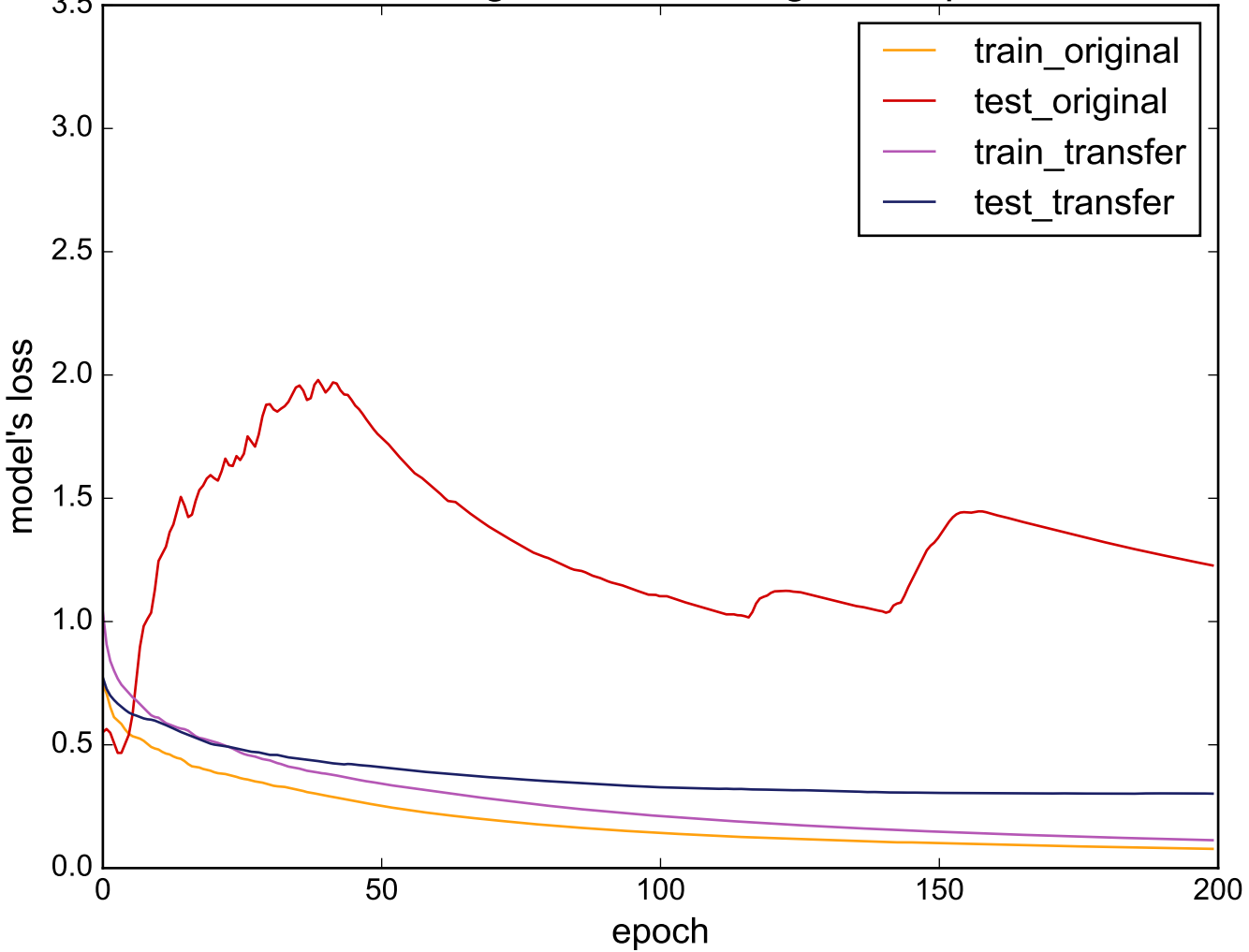
Source: StarLightCurves - Target: ShapeletSim
