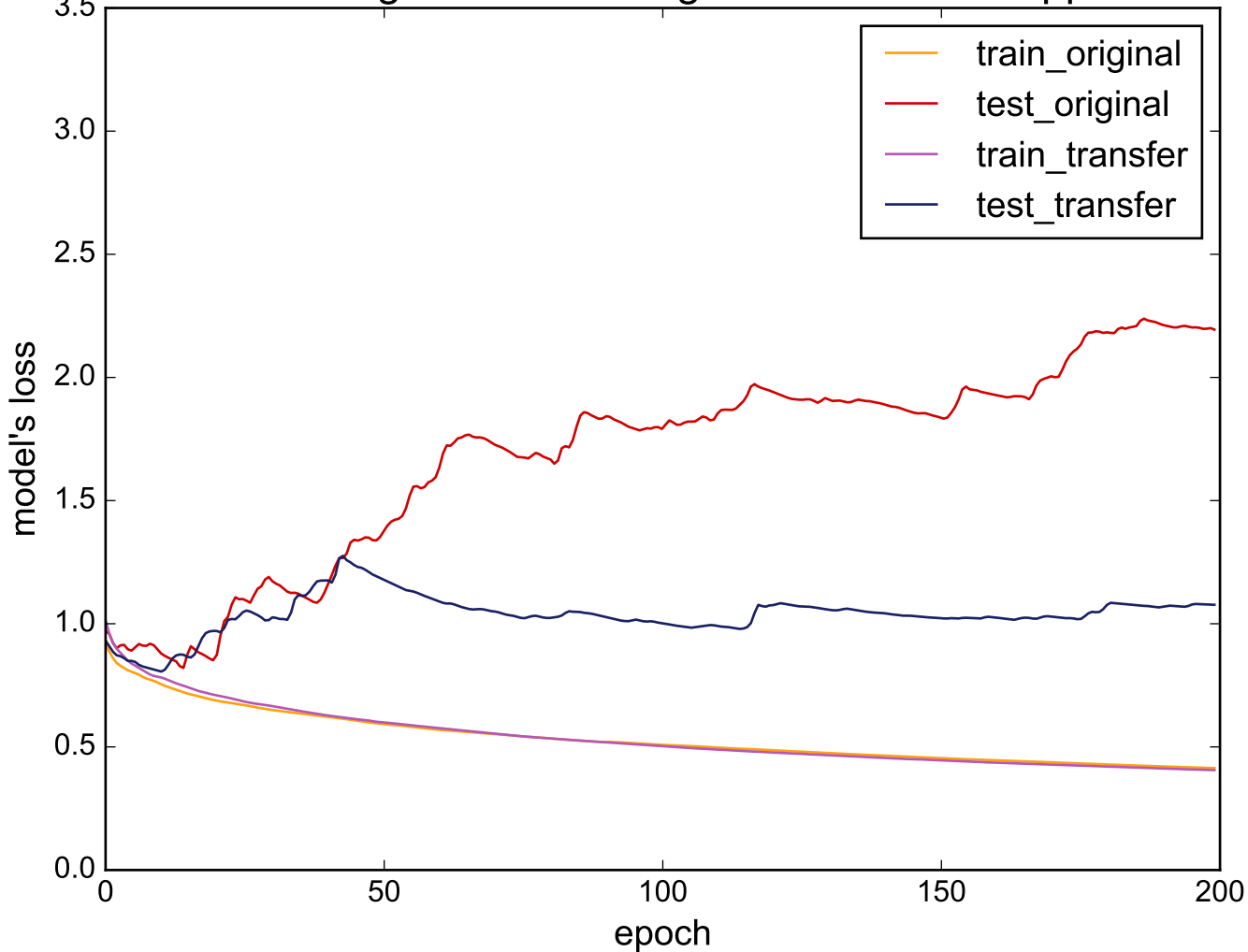
Source: StarLightCurves - Target: SmallKitchenAppliances
