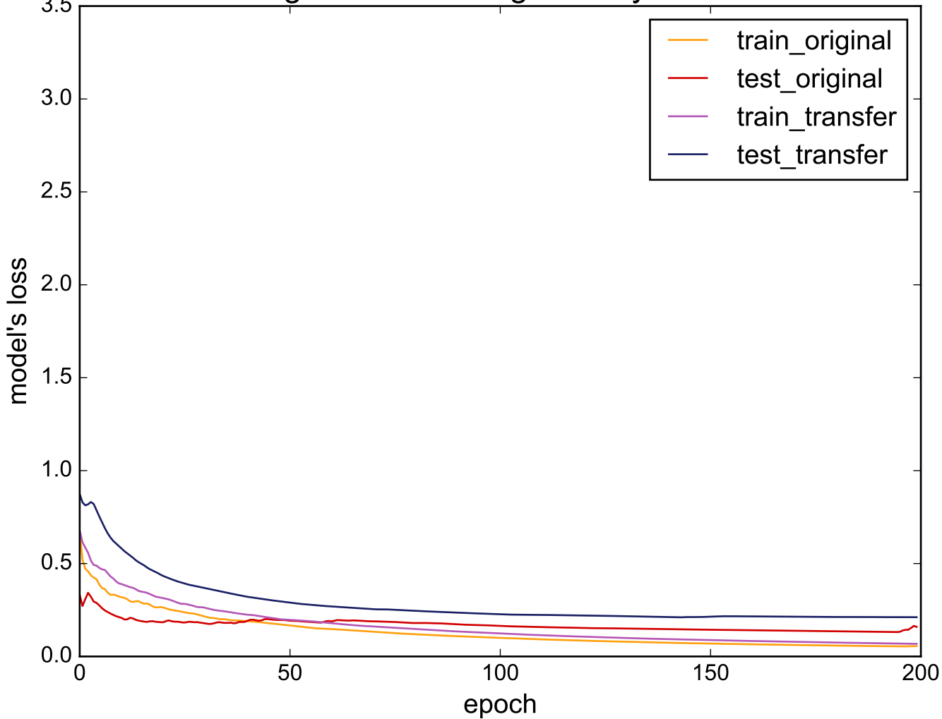
Source: StarLightCurves - Target: SonyAIBORobotSurface
