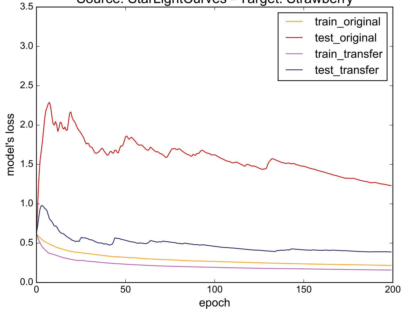
Source: StarLightCurves - Target: Strawberry
