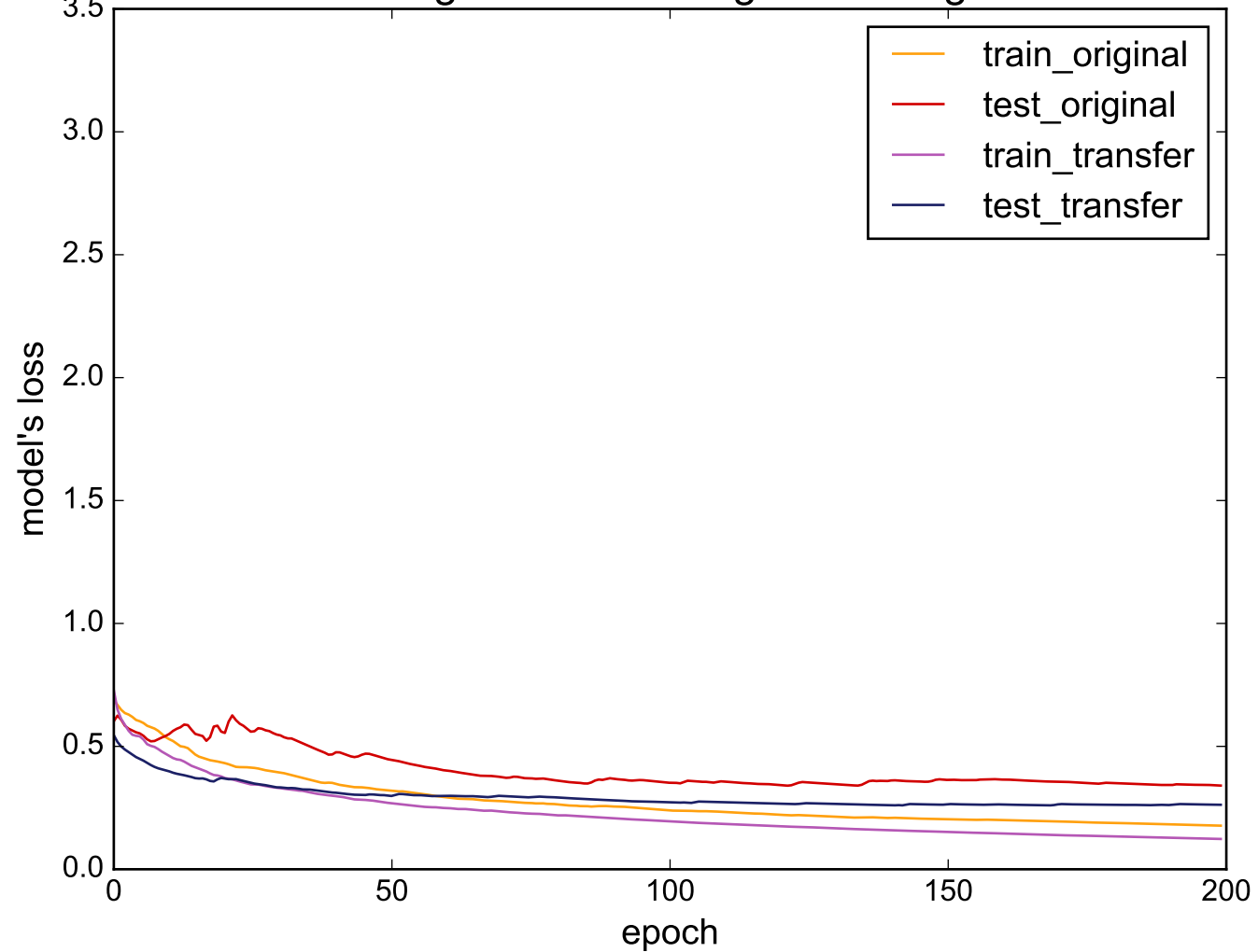
Source: StarLightCurves - Target: ToeSegmentation1
