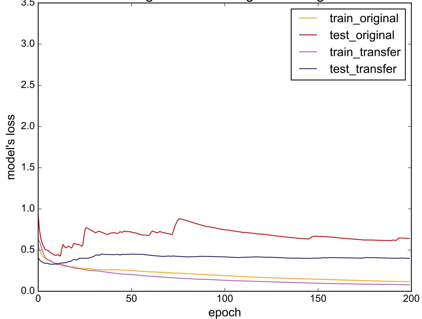
Source: StarLightCurves - Target: ToeSegmentation2
