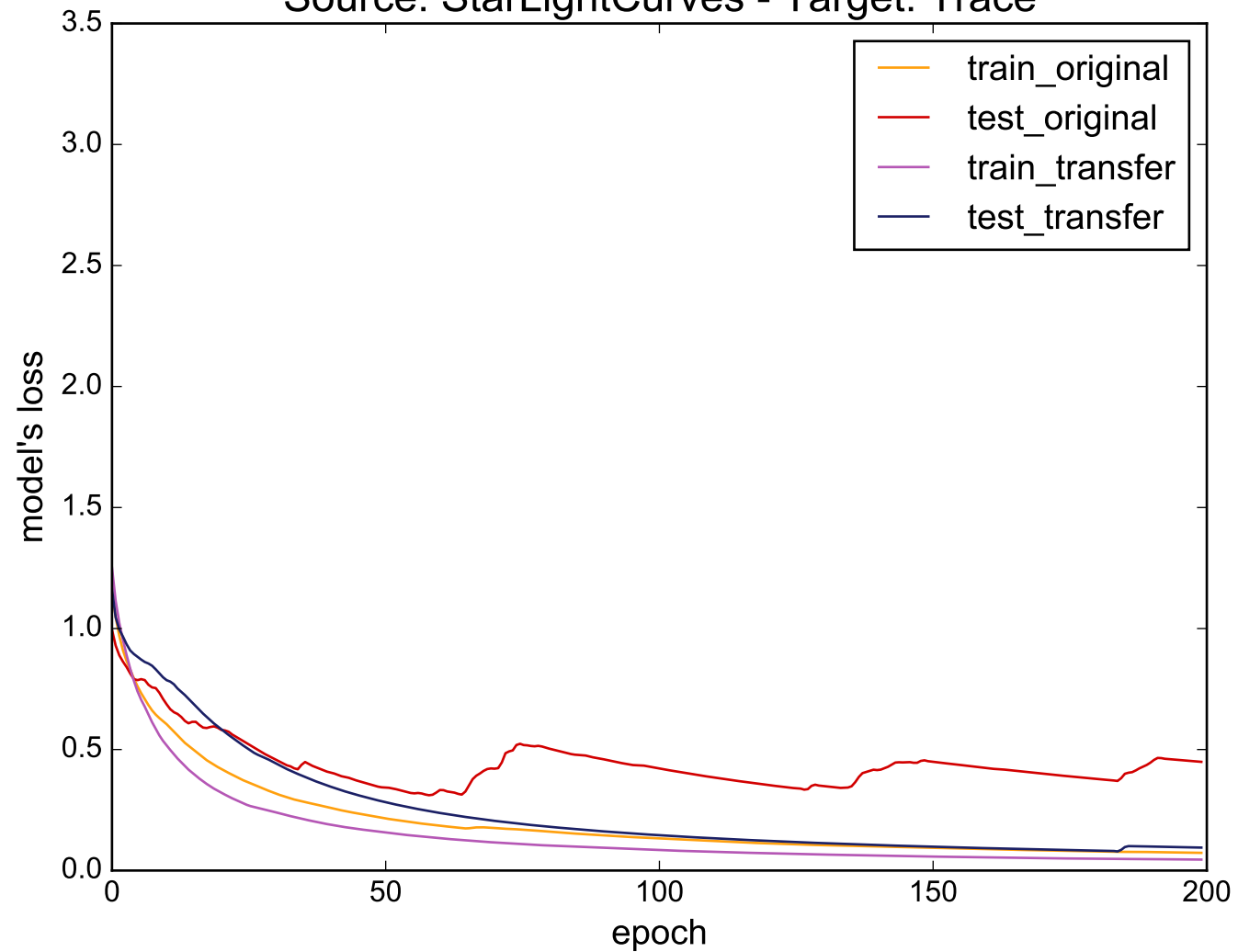
Source: StarLightCurves - Target: Trace
