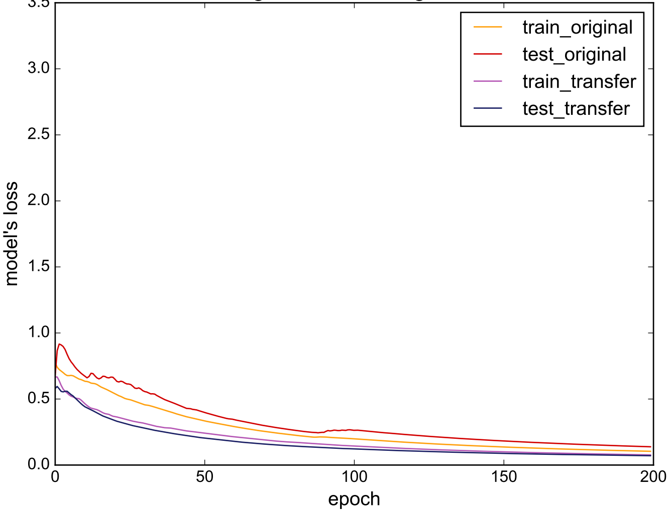
Source: StarLightCurves - Target: TwoLeadECG
