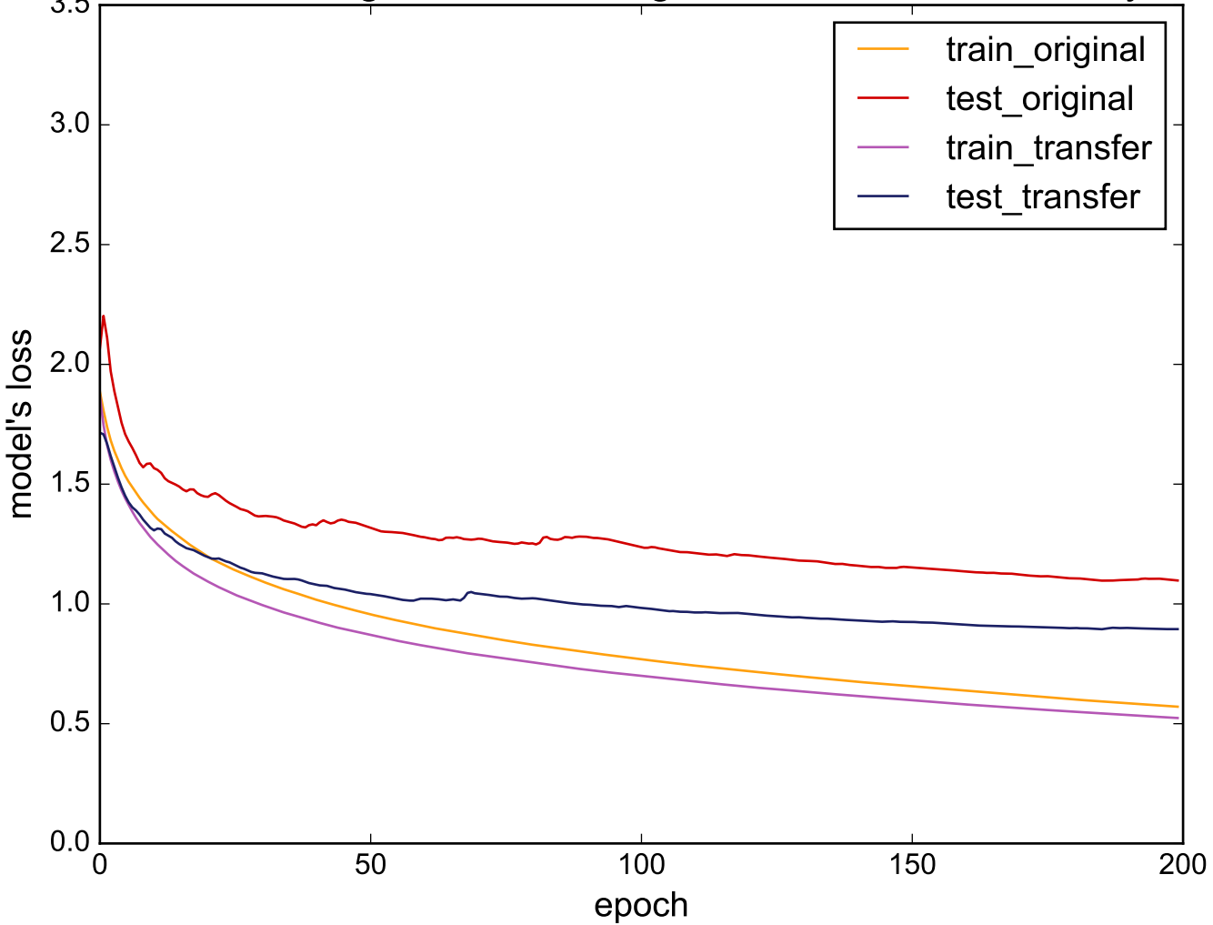
Source: StarLightCurves - Target: UWaveGestureLibraryAll
