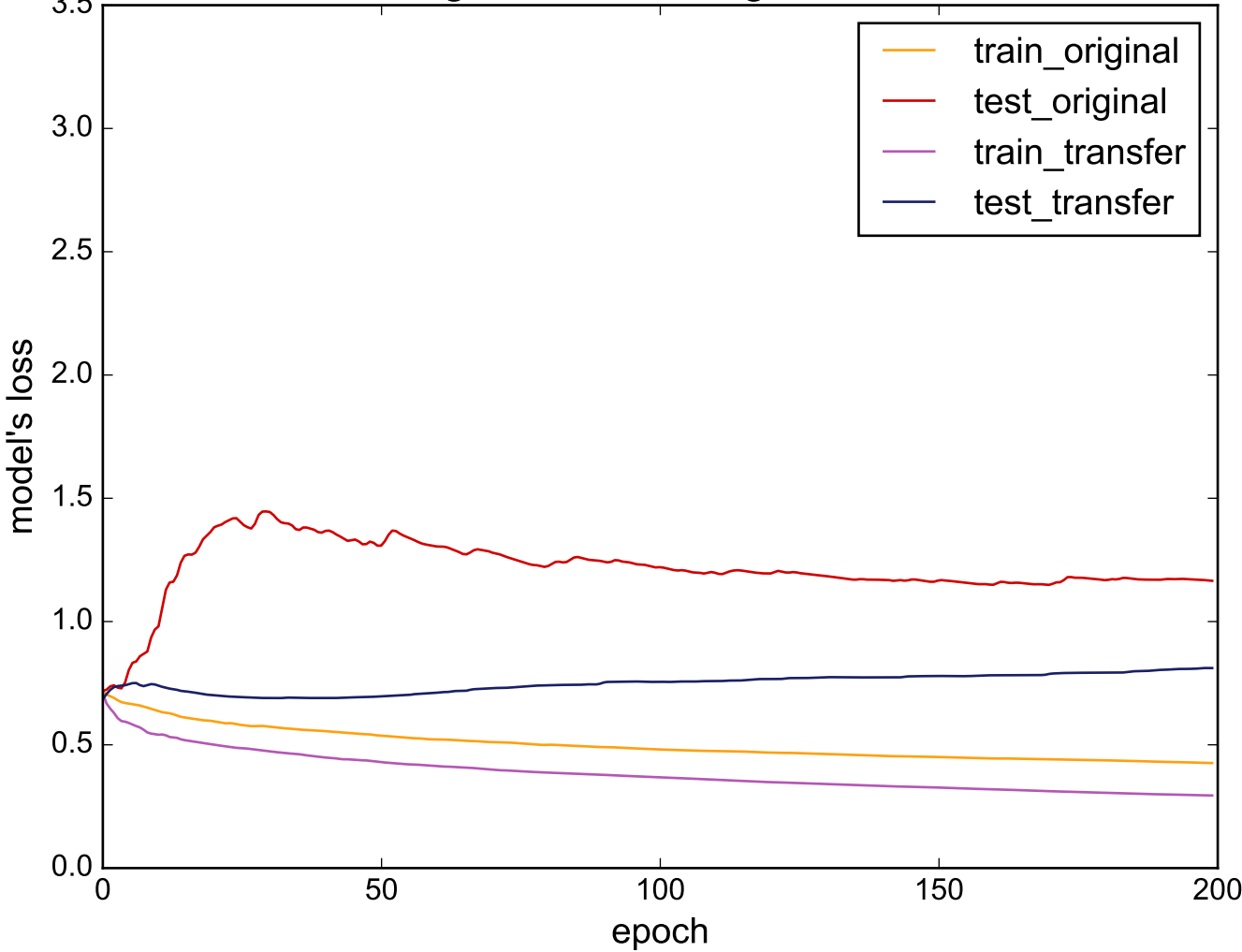
Source: StarLightCurves - Target: WormsTwoClass
