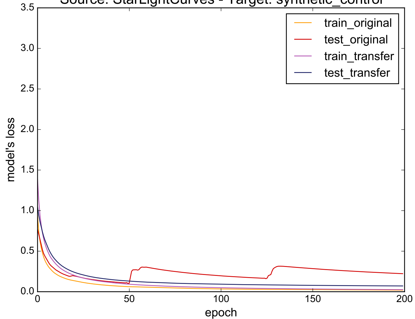
Source: StarLightCurves - Target: synthetic_control
